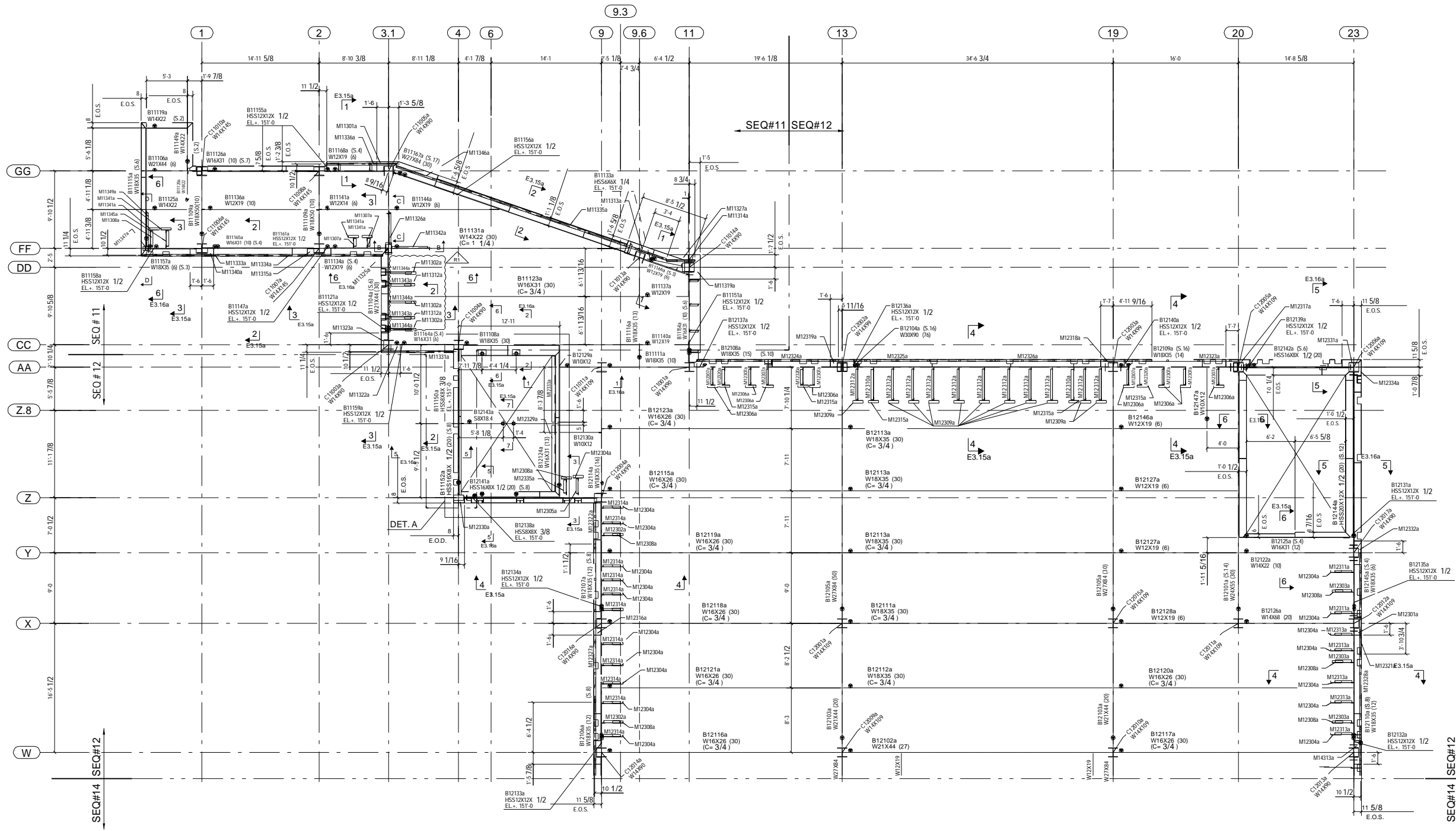
FOURTH FLOOR FRAMING PLAN T.O.S. EL. + 156'-6 1/2 U.N.O.
